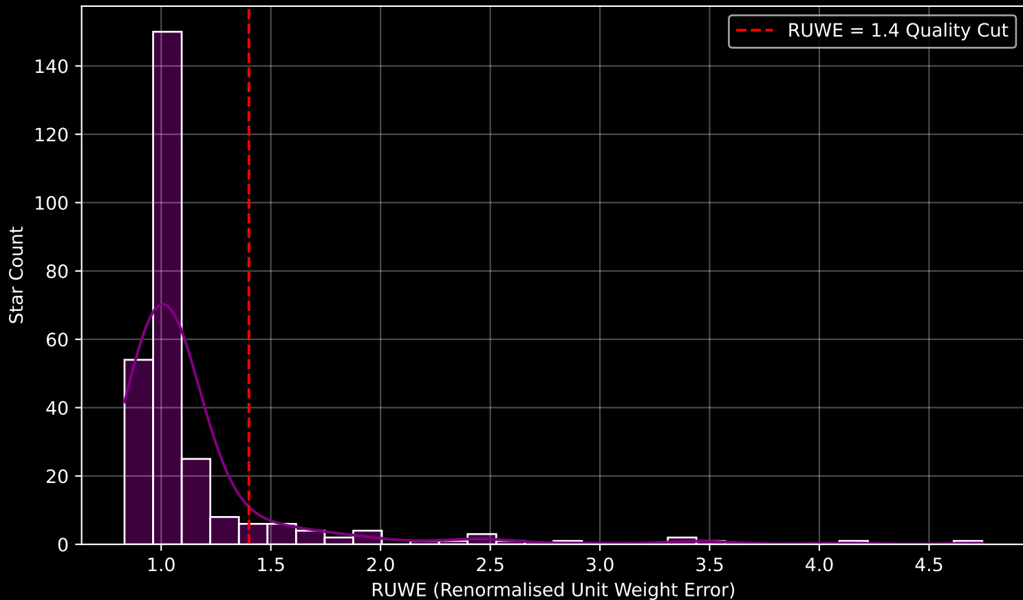
GALAH DR4 Field [826] RUWE Distribution (n= 271)
