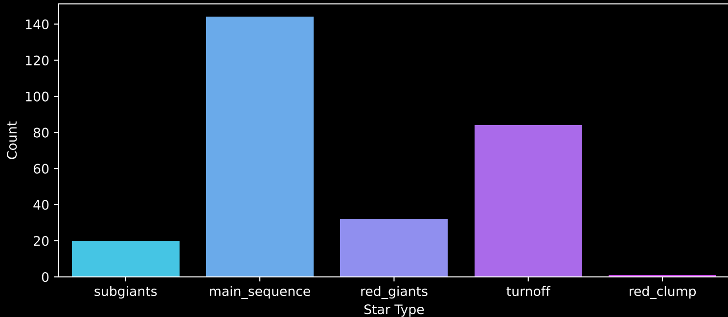
GALAH DR4 Field: [826] Count plot of Star Type
