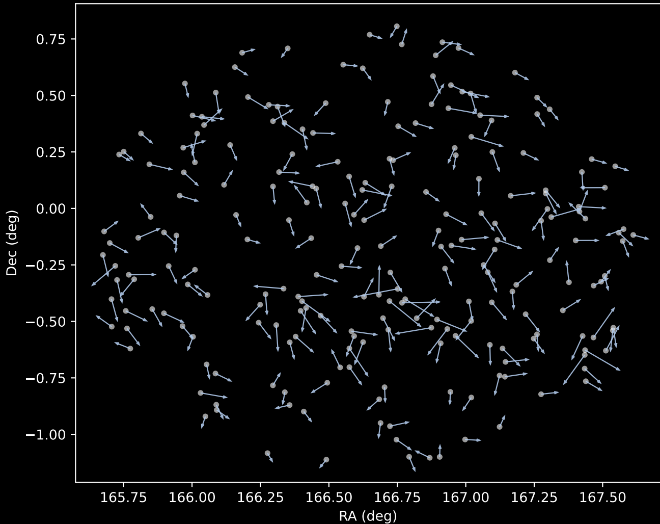
GALAH DR4 Cluster 1 Proper Motion Vectors (n=222)
